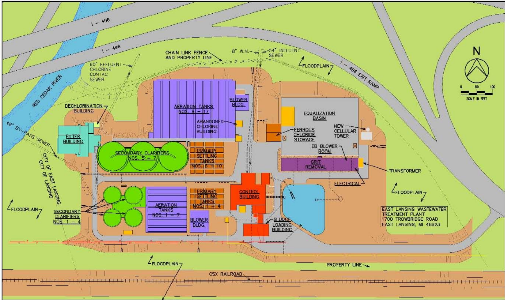
Figure 1-1: City of East Lansing WWTP Existing Site Plan
