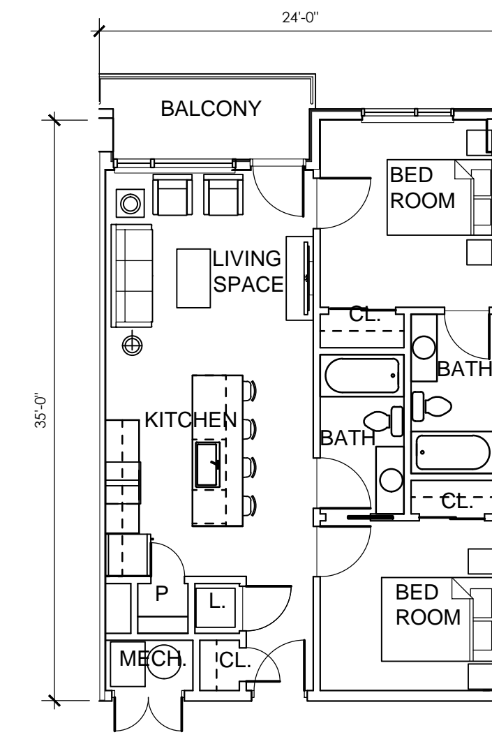
TYPICAL 2 BED UNIT 1" = 8'-0" 860 SQ. FT.
