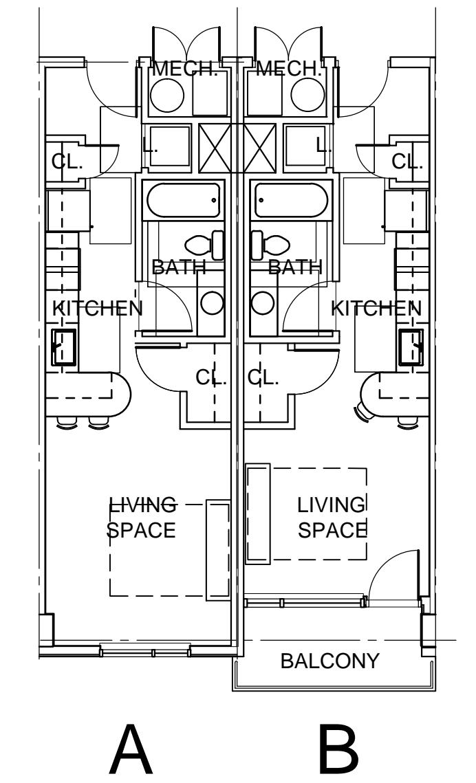
STUDIO UNITS 1" = 8'-0" A = 432 SQ. FT. B = 396 SQ. FT. Balcony = 60 SQ. FT.
