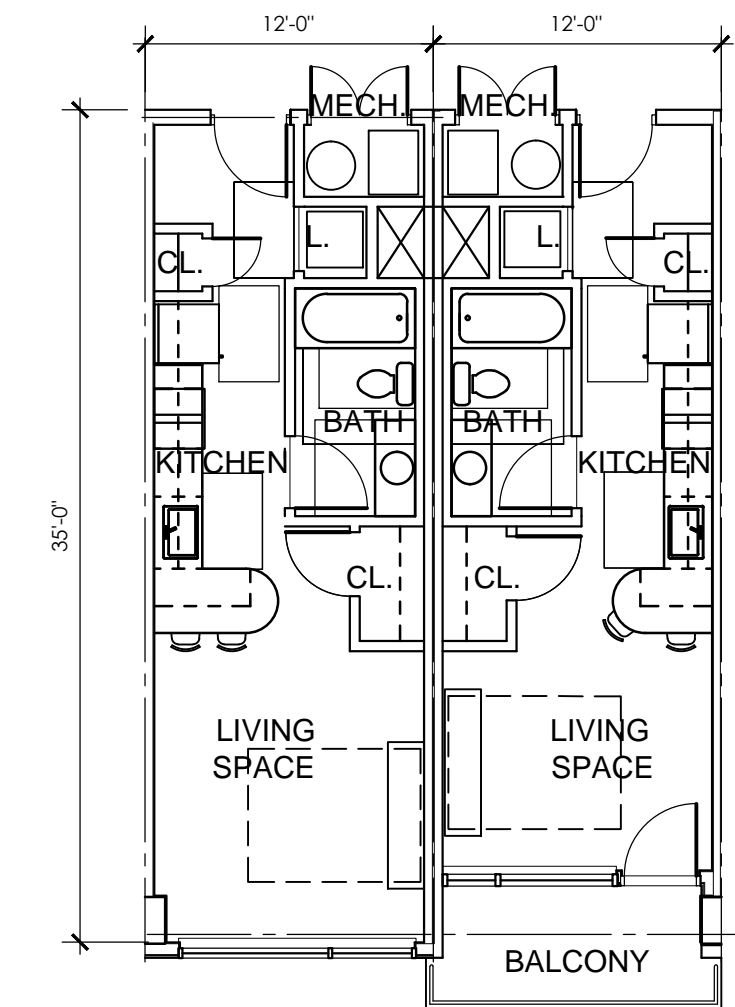
TYPICAL STUDIO UNITS 1" = 8'-0" 860 SQ. FT.
