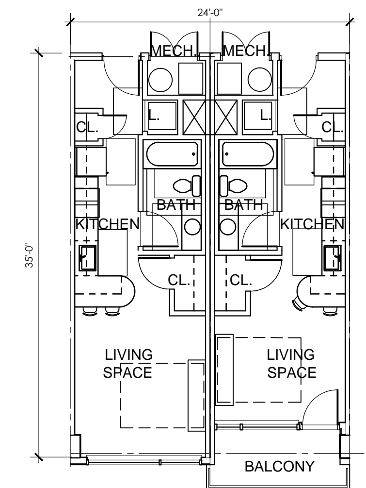
A B TYPICAL STUDIO UNITS
