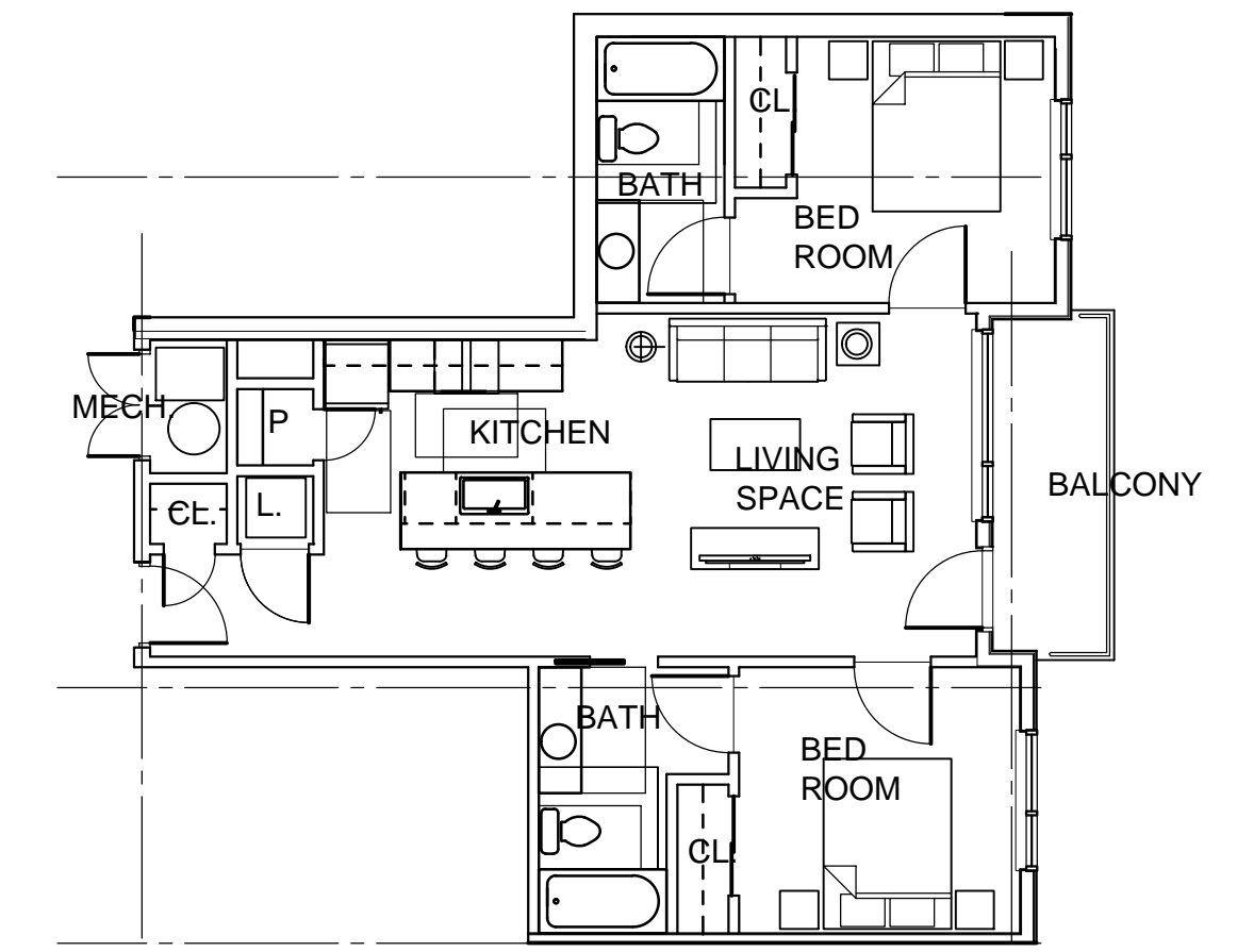
2 BED UNIT- TYPE 2 1" = 8'-0" 856 SQ. FT.
