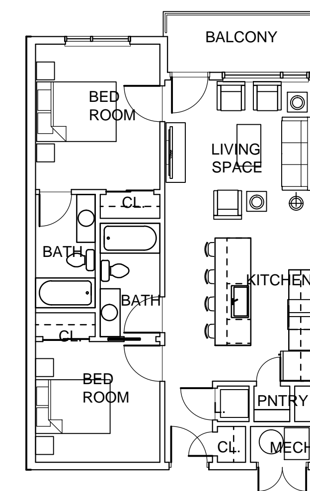
TWO BEDROOM UNITS 1" = 8'-0" 900 SQ. FT.
