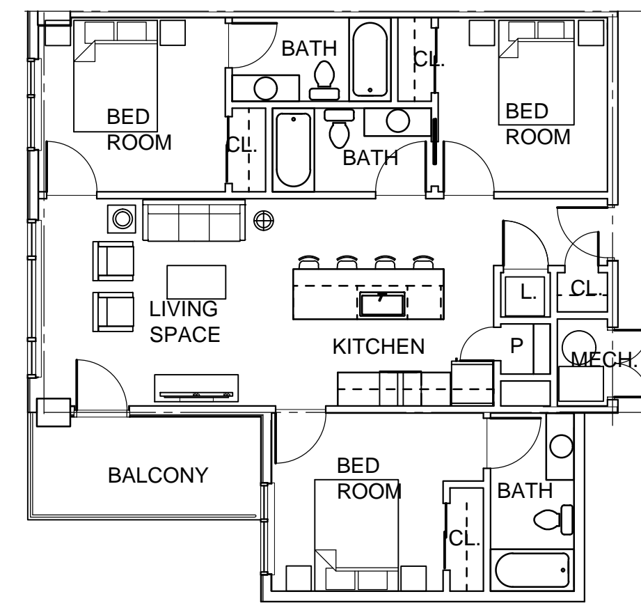
3 BED UNIT-TYPE 3 1" = 8'-0" 1200 SQ. FT.
