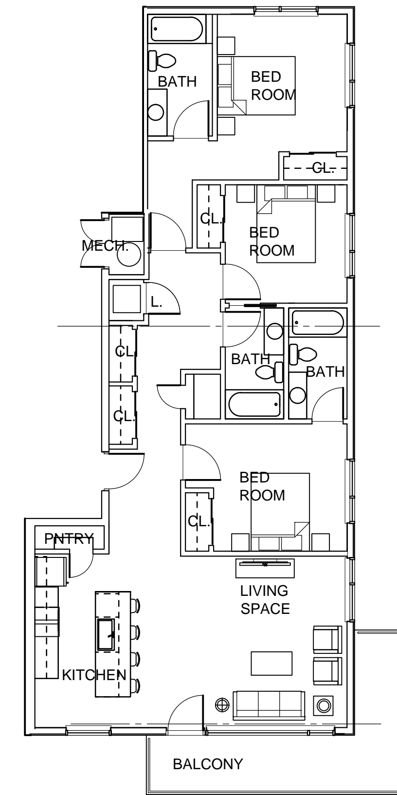
THREE BEDROOM UNIT 2 1" = 8'-0" 1500 SQ. FT.
