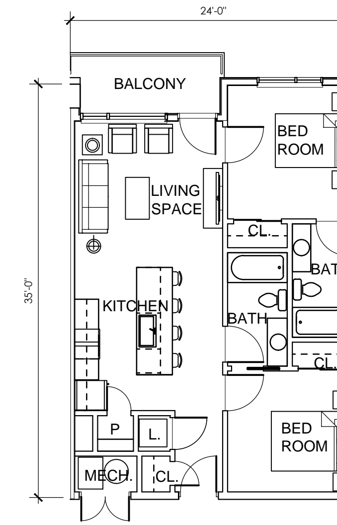
TYPICAL 2 BED UNIT 1" = 8'-0" 860 SQ. FT.
