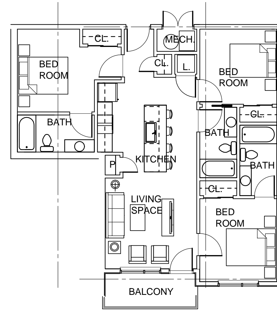
3 BED UNIT-TYPE 2 1" = 8'-0" 1075 SQ. FT.
