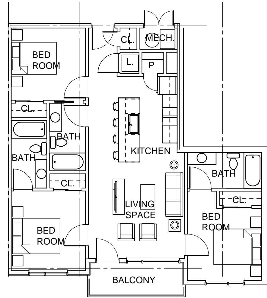
3 BED UNIT-TYPE 1 1" = 8'-0" 1100 SQ. FT.
